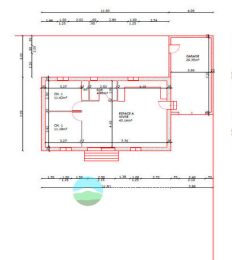
PLAN Ech. 1/100
